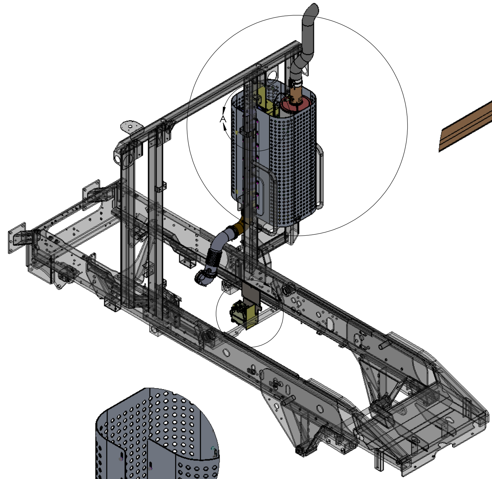
SCR, EXHAUST STACK, & BRACKETS PAGE 2
