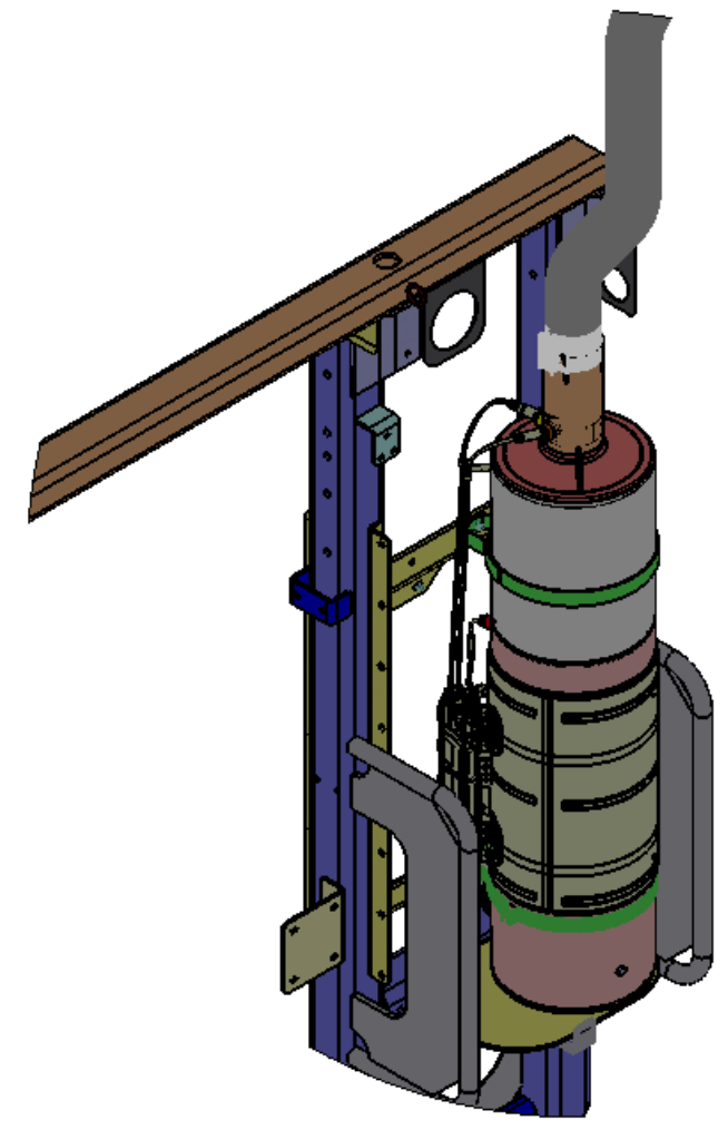
SCR, EXHAUST STACK, & BRACKETS PAGE 2
