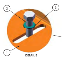
DETAIL E SCALE 1 : 1
