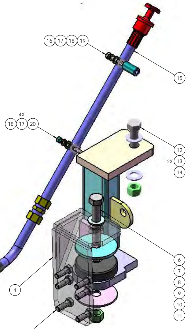
DETAIL A SCALE 2 : 5
