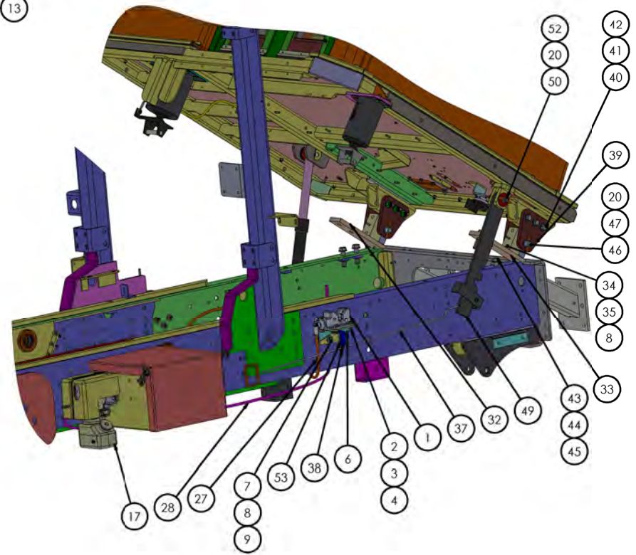
RIGHT VIEW
