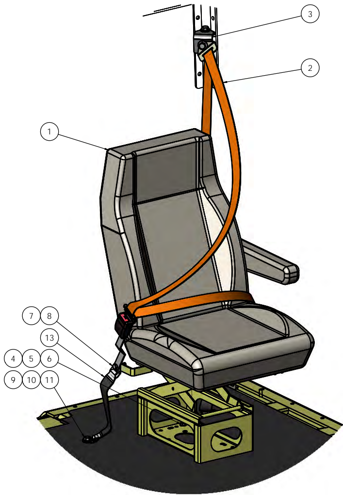
SEAT DETAIL
