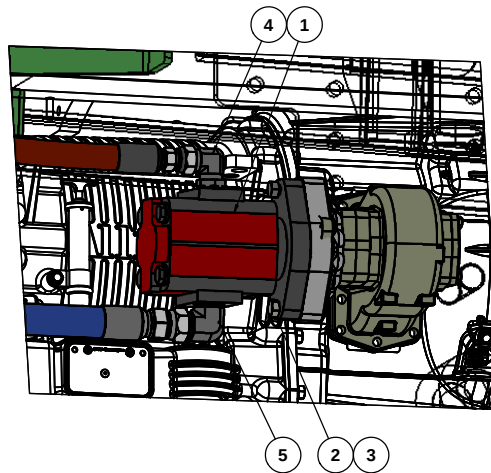
HYDRAULIC PUMP
