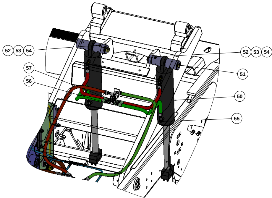
CYLINDER VIEW
