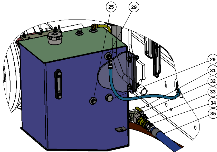
HYDRAULIC TANK FRONT VIEW
