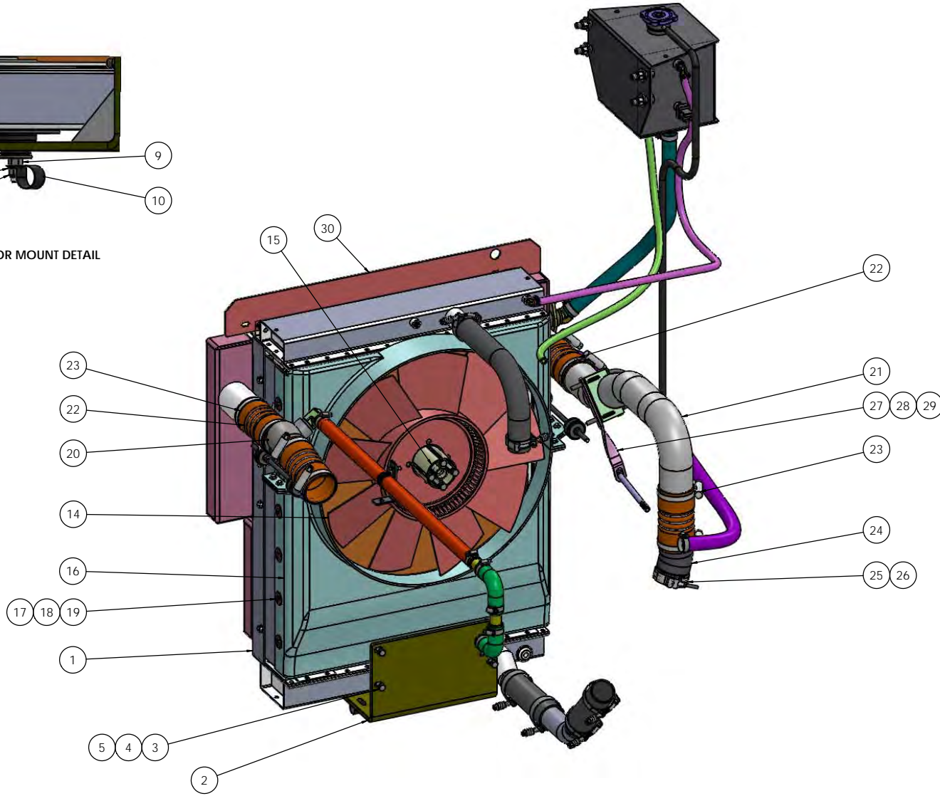
RADIATOR DETAIL & CAC TUBES
