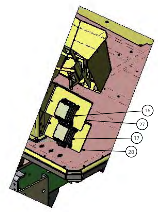
ELECTRICAL MODULES
