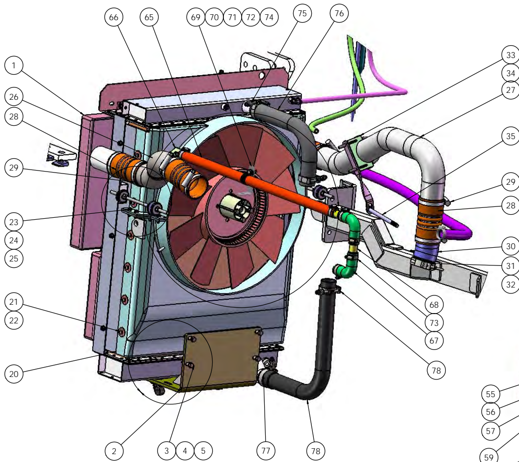
RADIATOR ASSEMBLY
