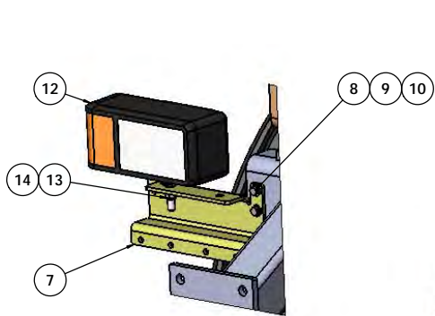
RH HEADLIGHT ASSEMBLY
