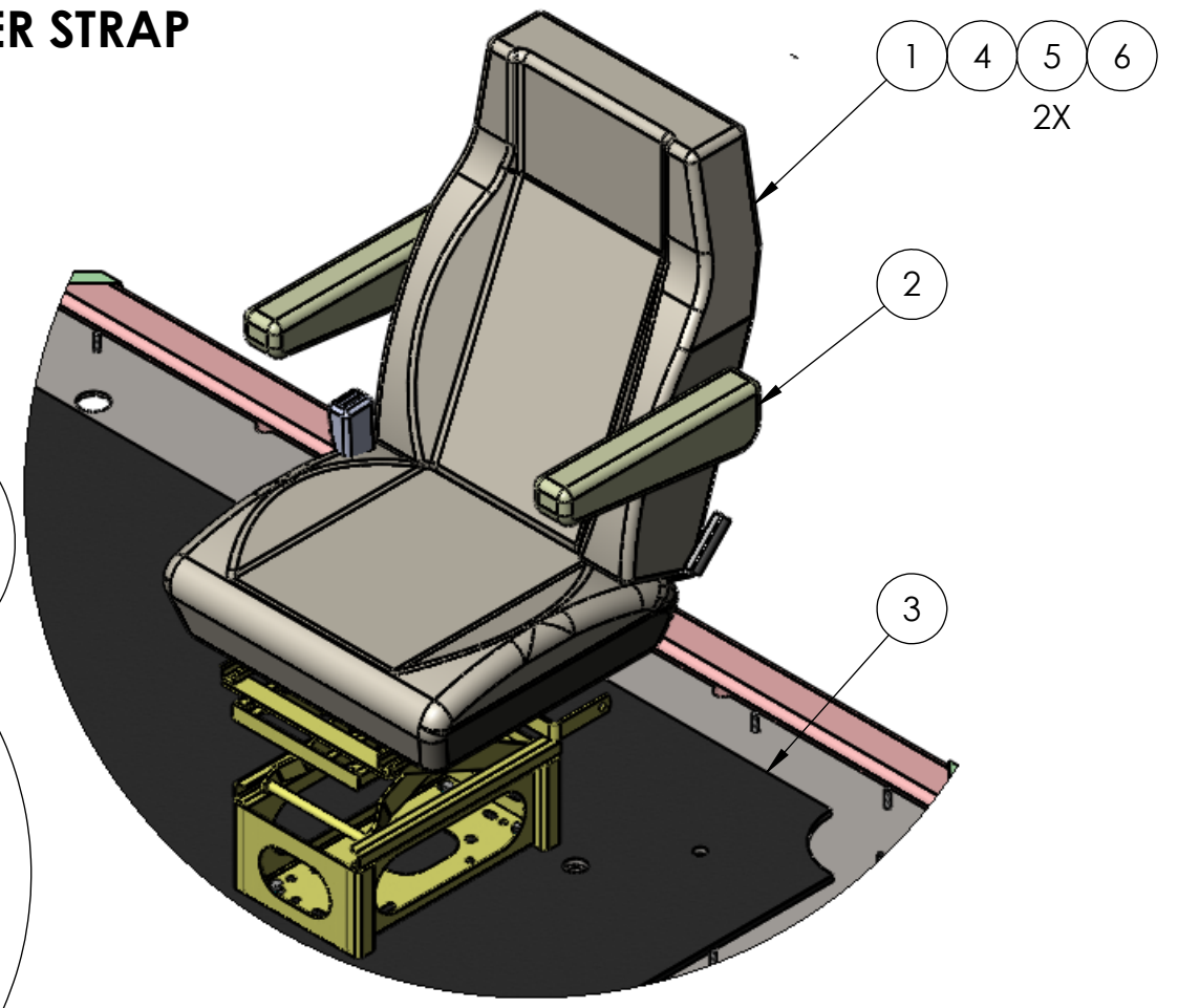
SEAT & FLOOR
