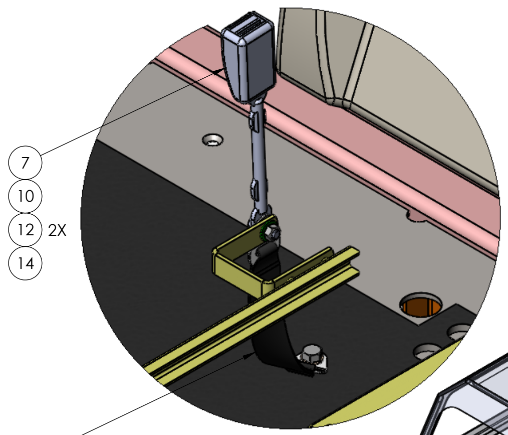
SEAT BELT & TETHER
