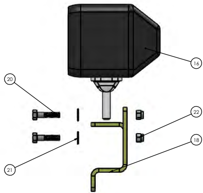
LH HEADLIGHT
