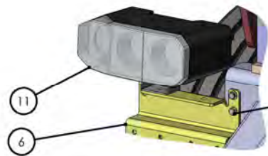
RH HEADLIGHT DETAIL
