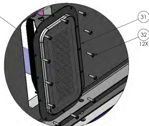
DETAIL D SCALE 1 : 3
