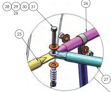
DETAIL E SCALE 1 : 2
