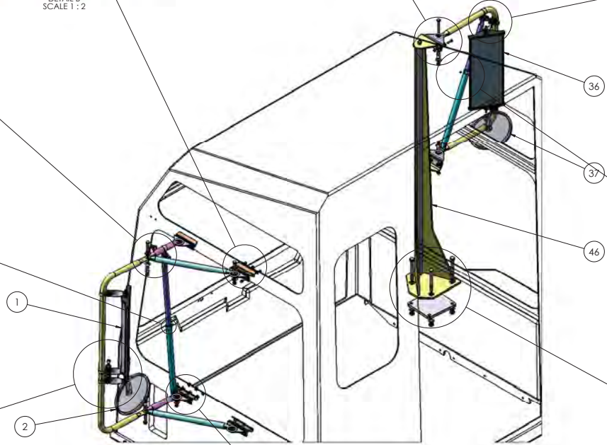
DETAIL B SCALE 1 : 2
