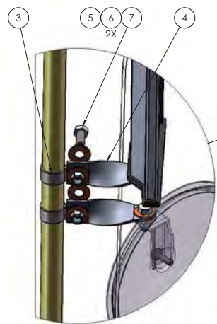
DETAIL A SCALE 1 : 2
