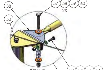
DETAIL G SCALE 1 : 3
