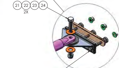
DETAIL AE SCALE 1 : 2
