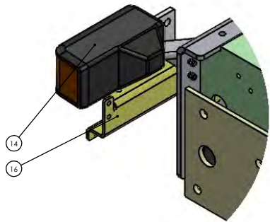
RH HEADLIGHT
