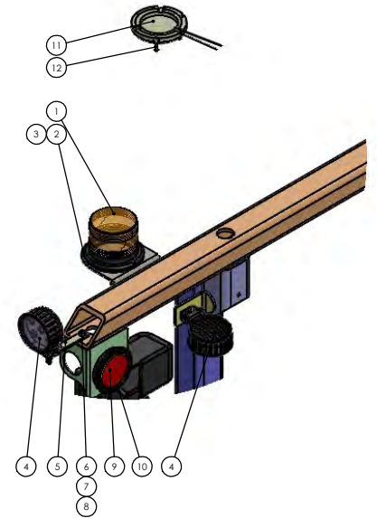
CAB BAR LIGHT CLUSTER
