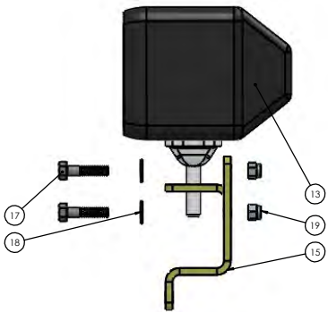
LH HEADLIGHT
