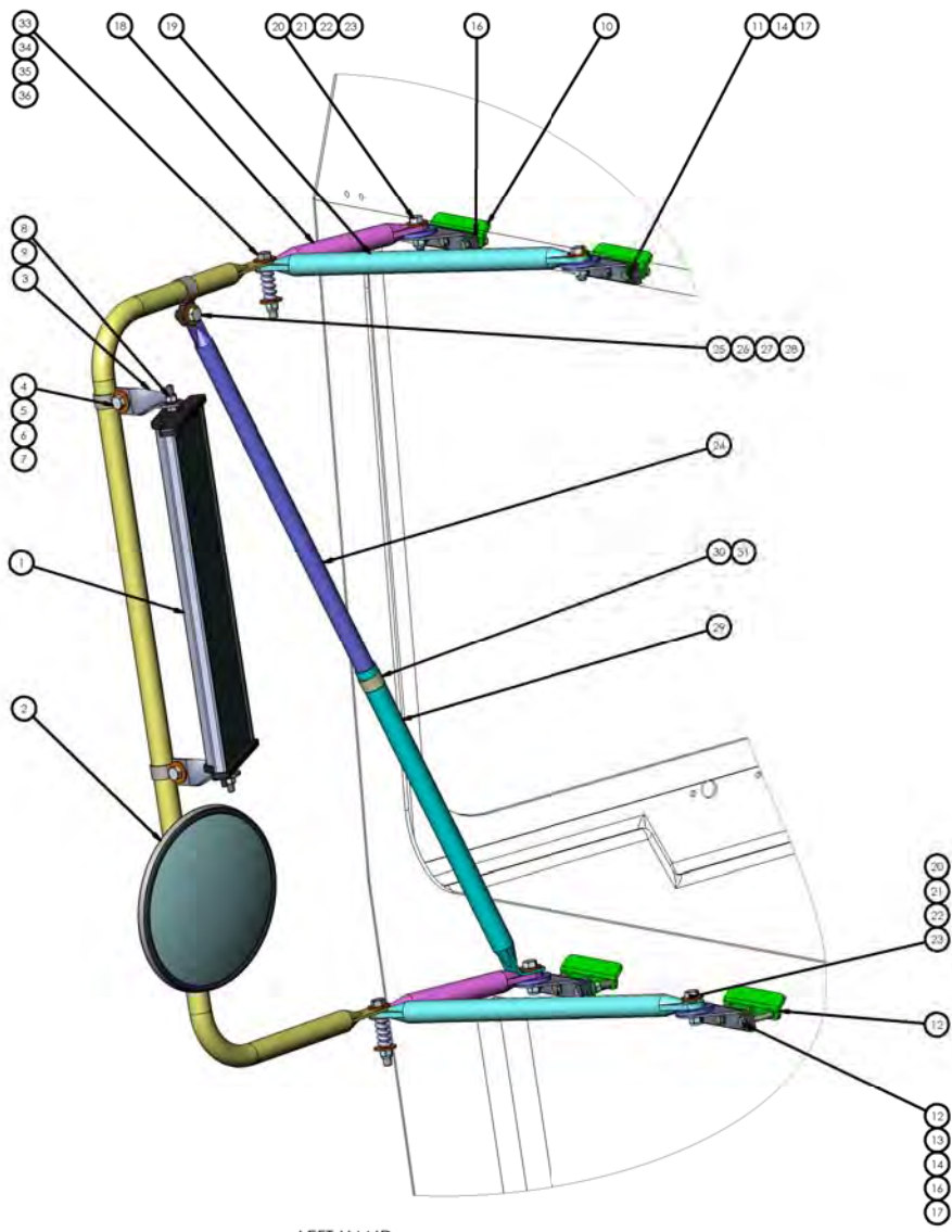
LEFT HAND MIRROR ASSEMBLY
