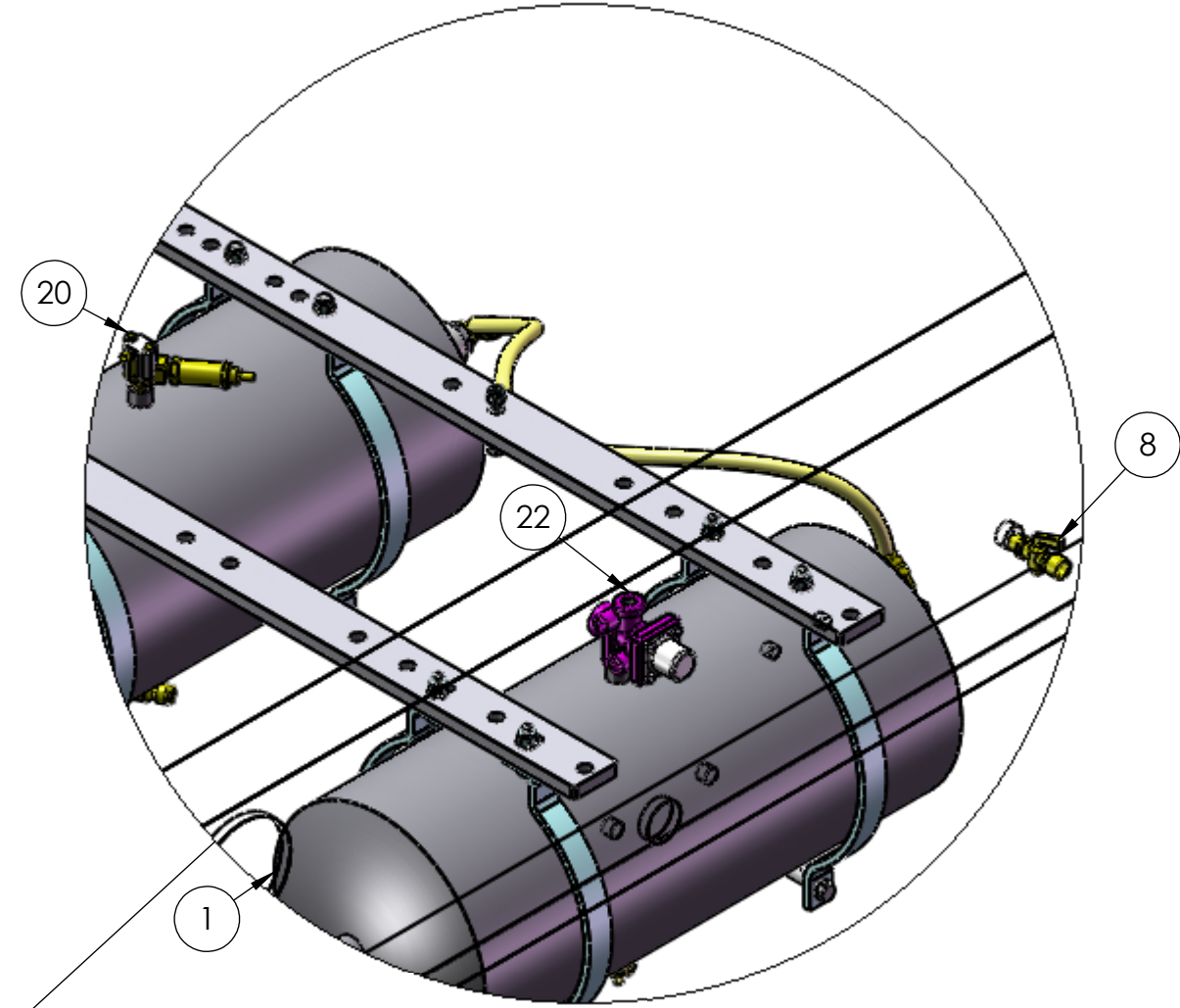
DETAIL C SCALE 1 : 6
