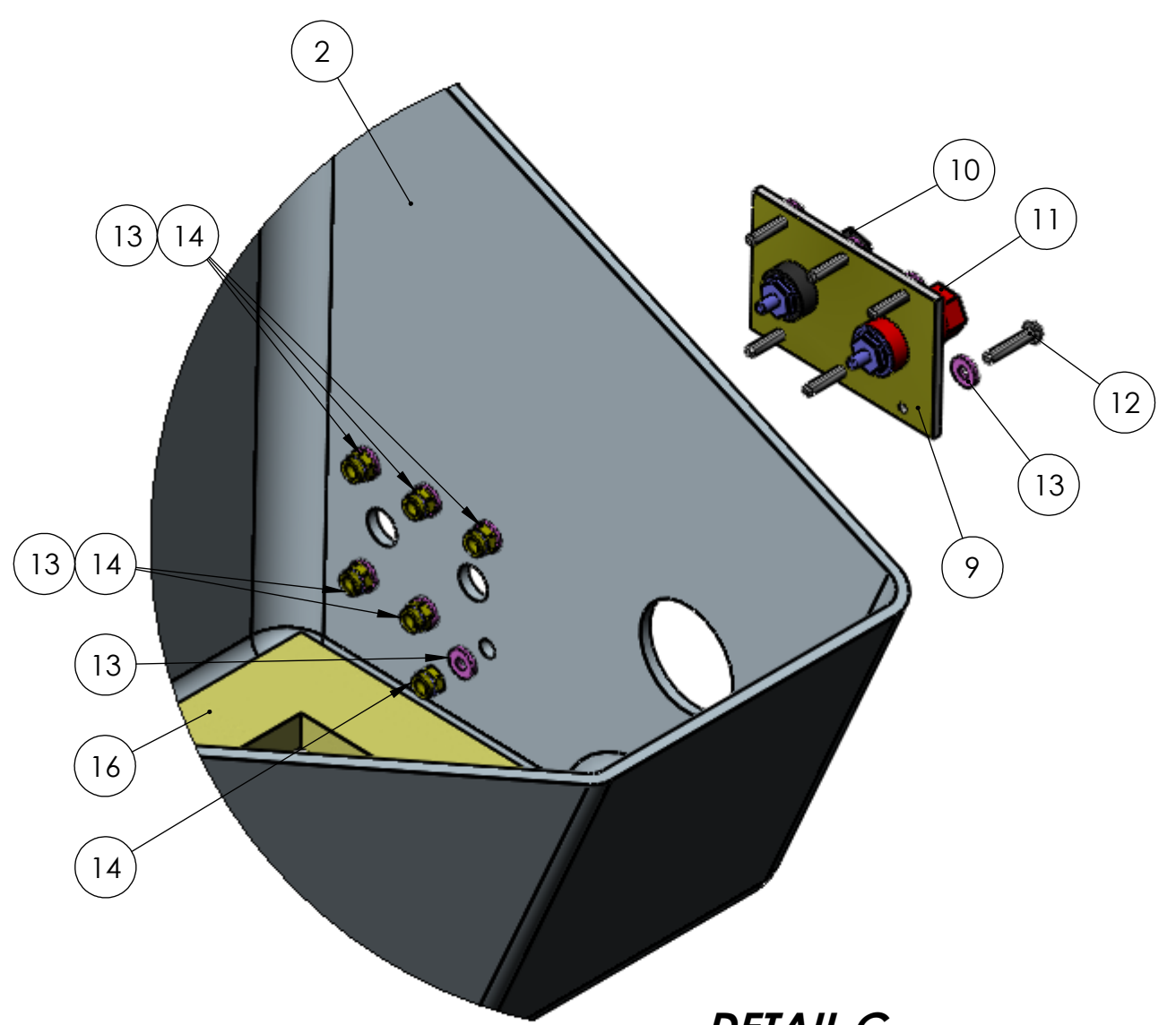
DETAIL C SCALE 1 : 2
