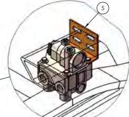
DETAIL E SCALE 1 : 3
