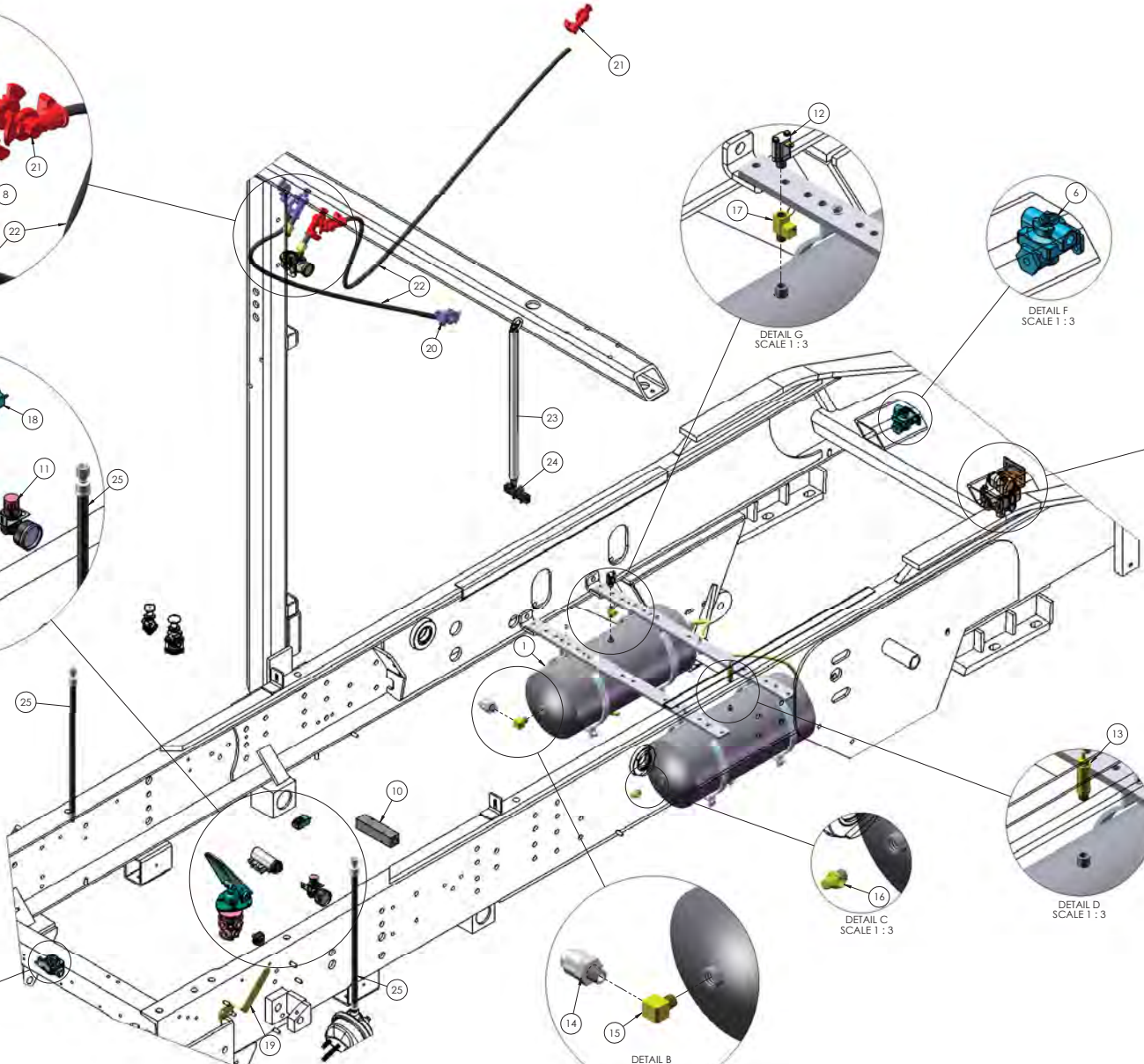
DETAIL B SCALE 1 : 3
