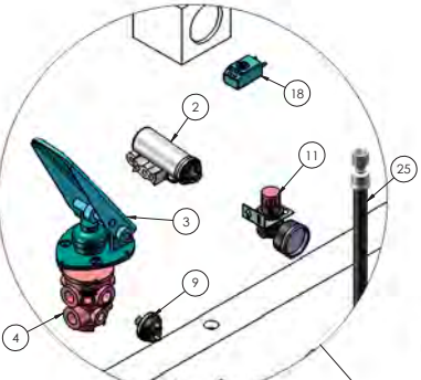
DETAIL I SCALE 1 : 4
